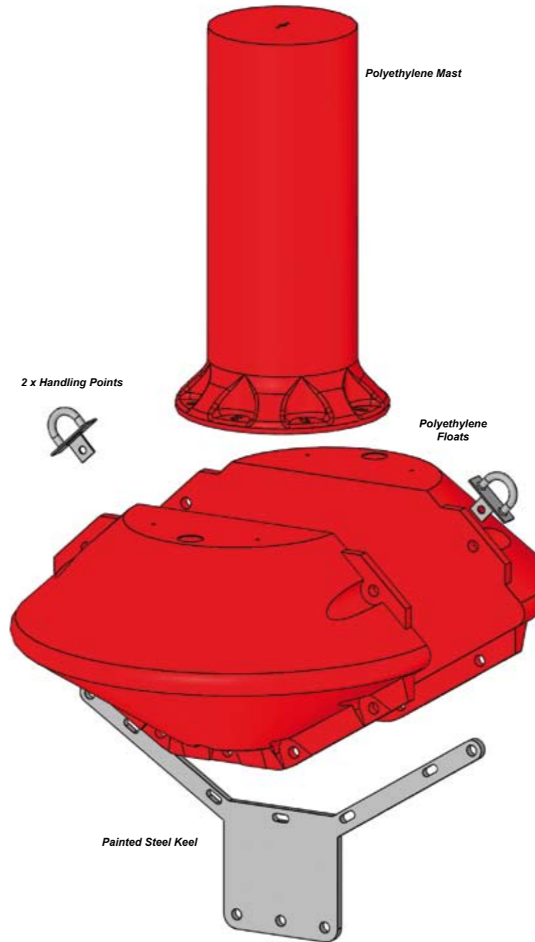
Exploded view of a MODULE 1200 Anchoring elements (shackles, chains, swivels, sinkers) are available in mooring device section in catalogue
